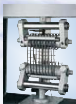
SF200 加勁格網 Tensile Grips for Anti- Erosion Netting
